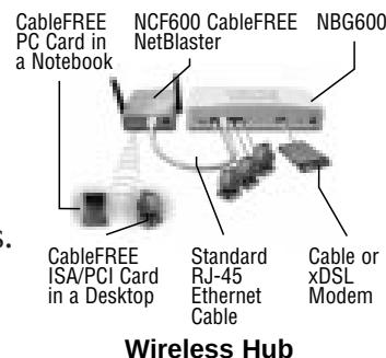
Wireless Hub
